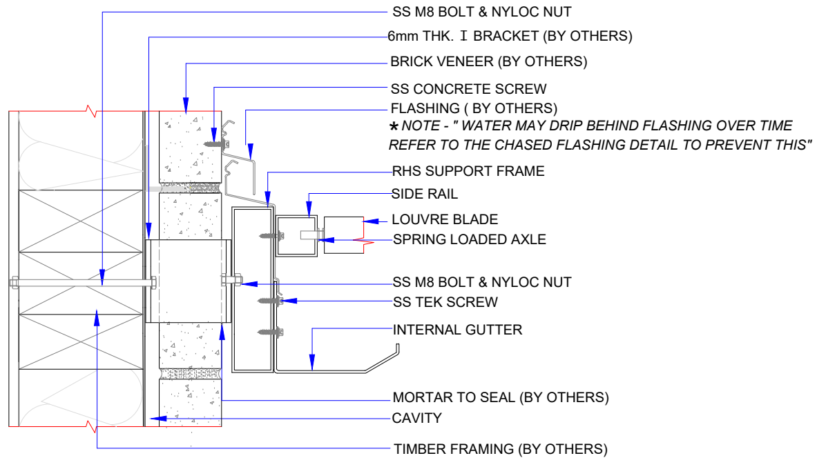
CROSS SECTION VIEW LOUVRE ROOF TO BRICK VENEER FIXING DETAILS
