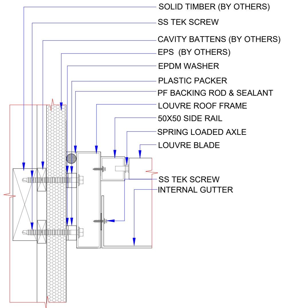
CROSS SECTION LOUVRE ROOF TO EPS FIXING DETAILS
