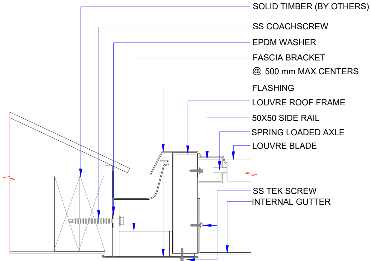
CROSS SECTION LOUVRE ROOF TO FASCIA BRACKET FIXING DETAILS
