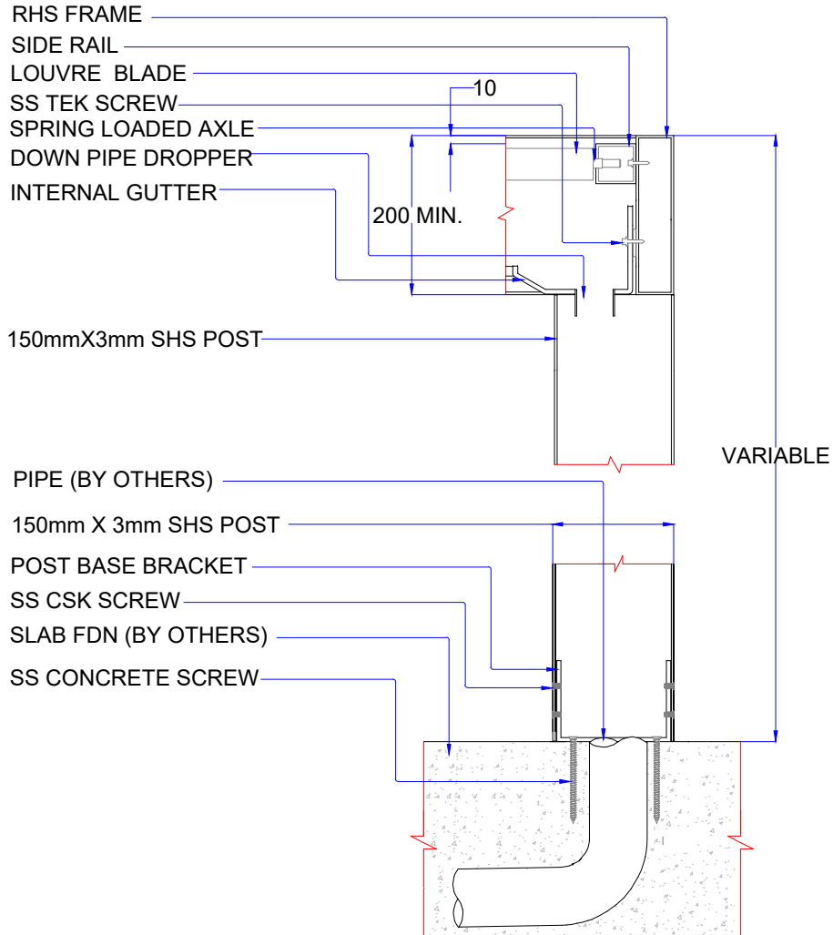
LOUVRE ROOF DRAINAGE INSIDE ALUMINIUM POST ELEVATION VIEW ( SECTION )
