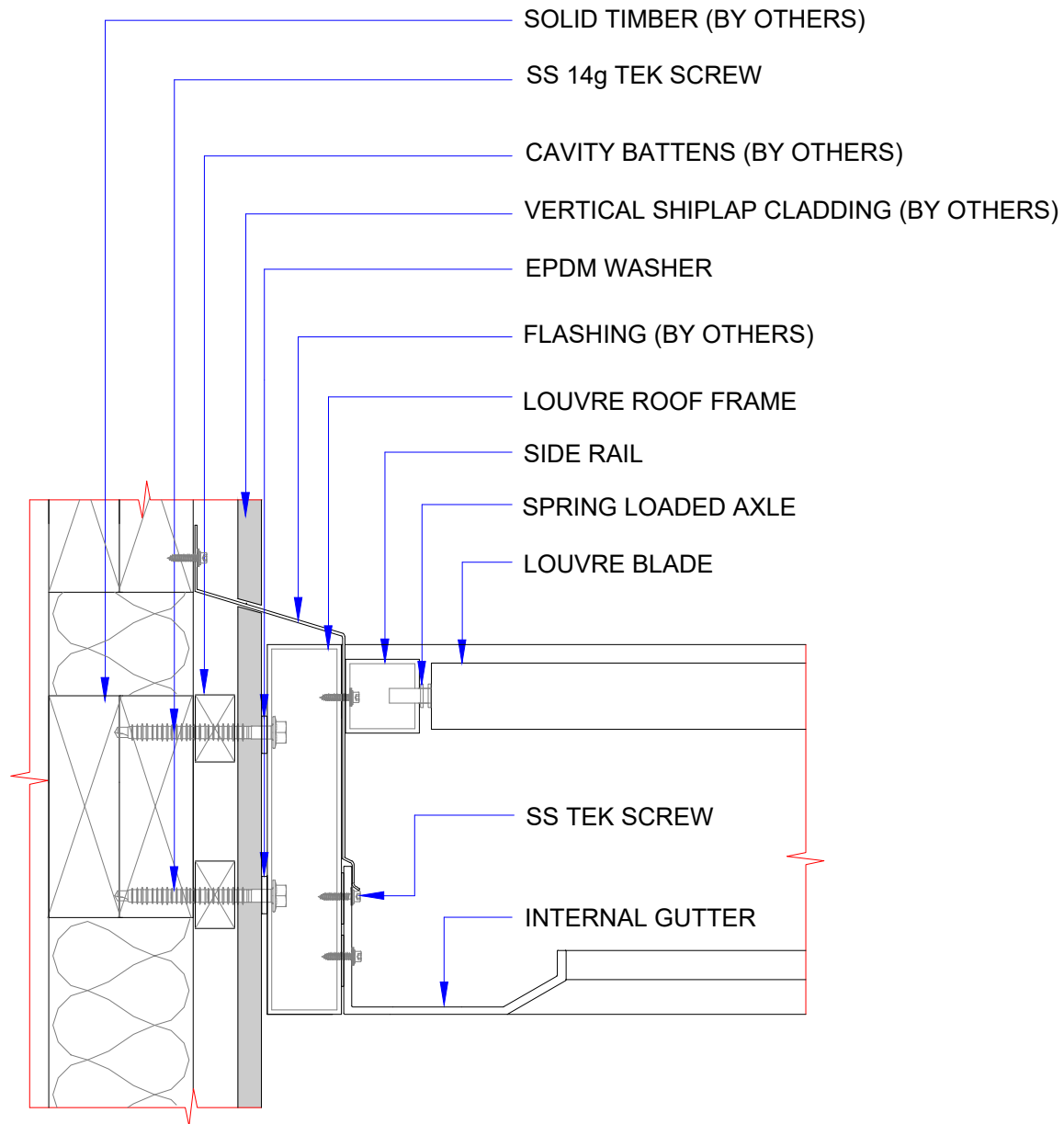
TYP. SIDE ELEVATION (SECTION) LOUVRE ROOF TO VERTICAL SHIPLAP FIXING DETAILS
