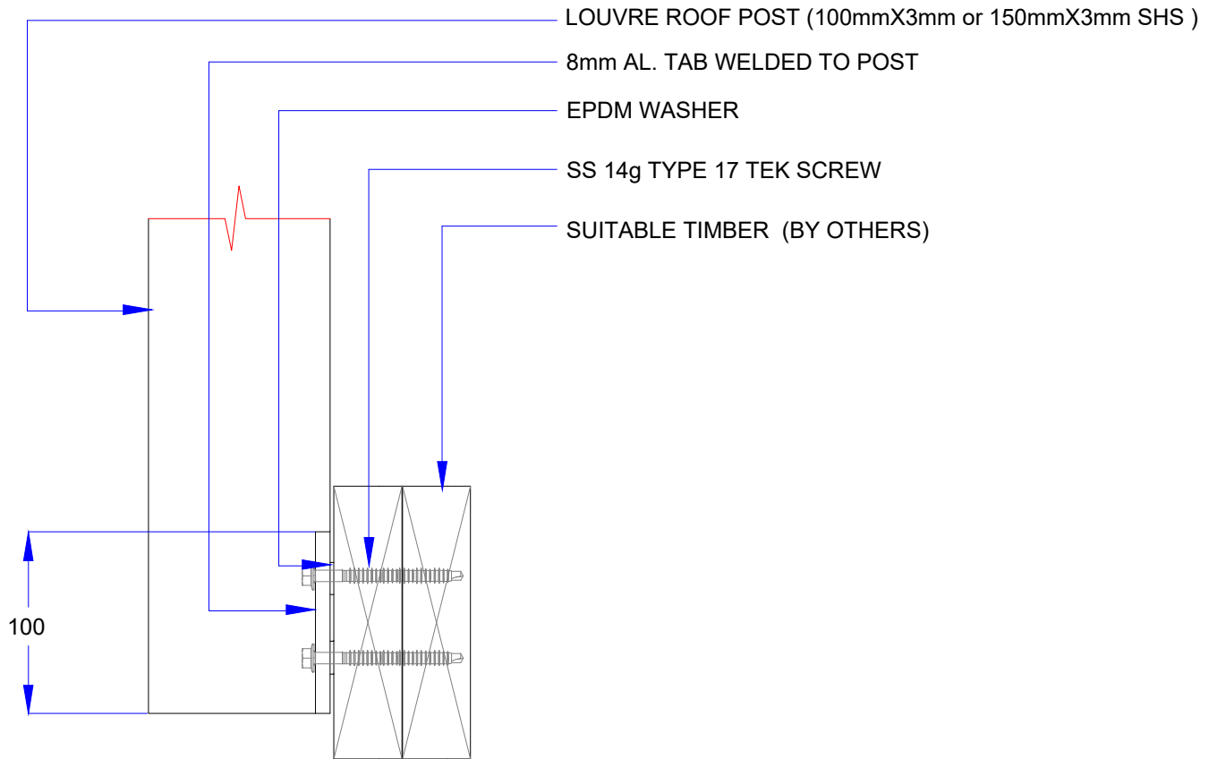
CROSS SECTION VIEW LOUVRE ROOF POST - DECK SIDE FIXING - CONNECTION DETAILS
