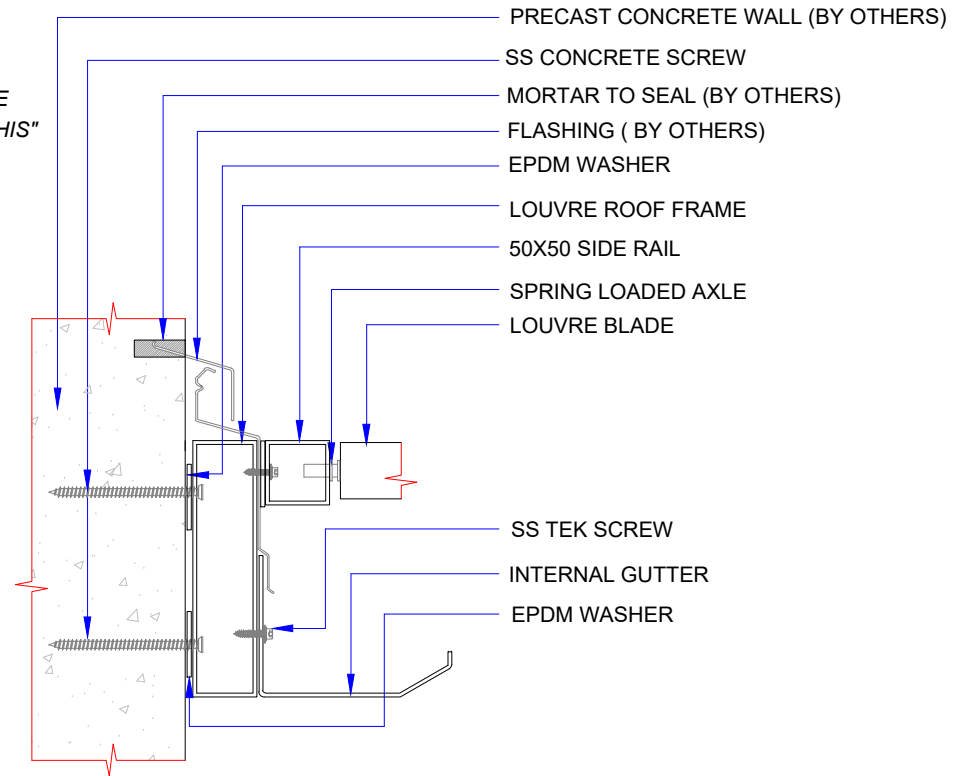
CROSS SECTION VIEW - ( CHASED FLASHING) LOUVRE ROOF TO PRECAST CONCRETE WALL FIXING DETAILS
