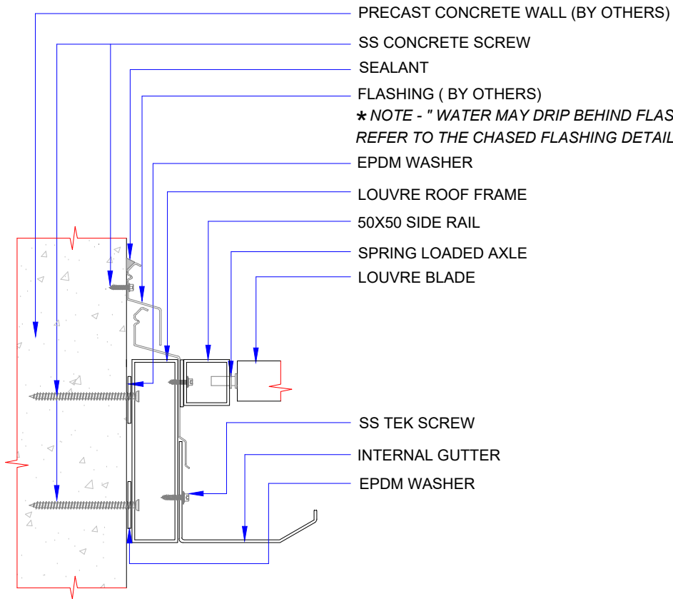
CROSS SECTION VIEW LOUVRE ROOF TO PRECAST CONCRETE WALL FIXING DETAILS
