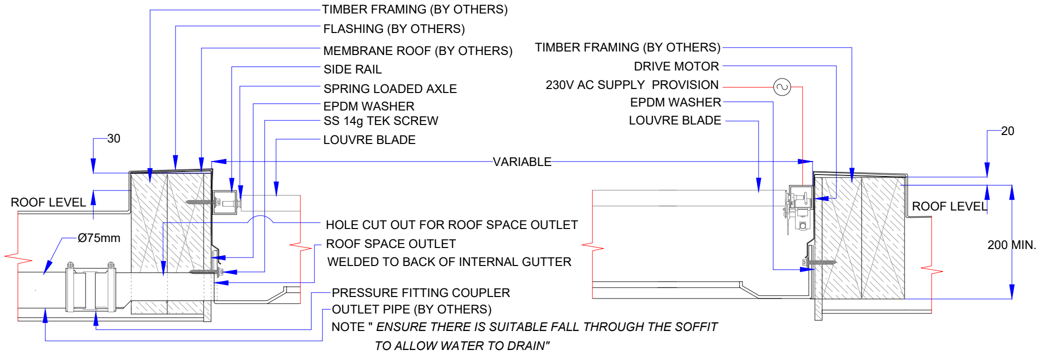
ELEVATION VIEW (LONGITUDINAL SECTION) OPENING ROOF (LOUVRE ROOF FIX TO TIMBER) * SHOWING REAR EXIT GUTTER
