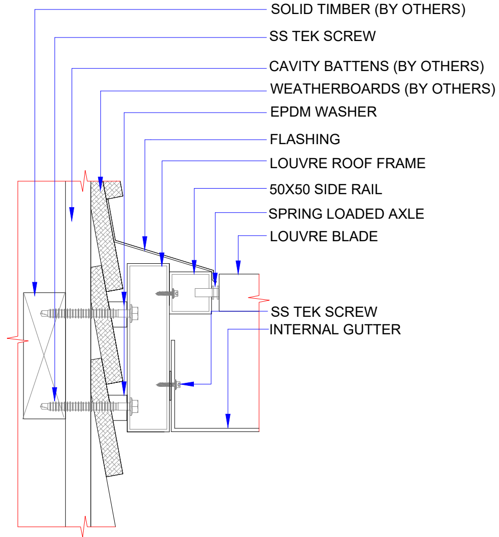
CROSS SECTION LOUVRE ROOF TO WEATHERBOARDS FIXING DETAILS
