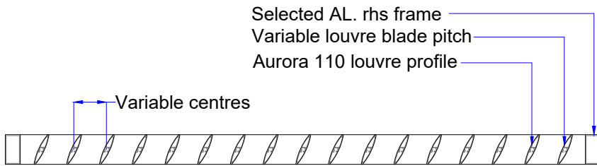
Plan view (section)
