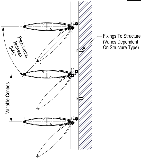
SECTIONED VIEW
