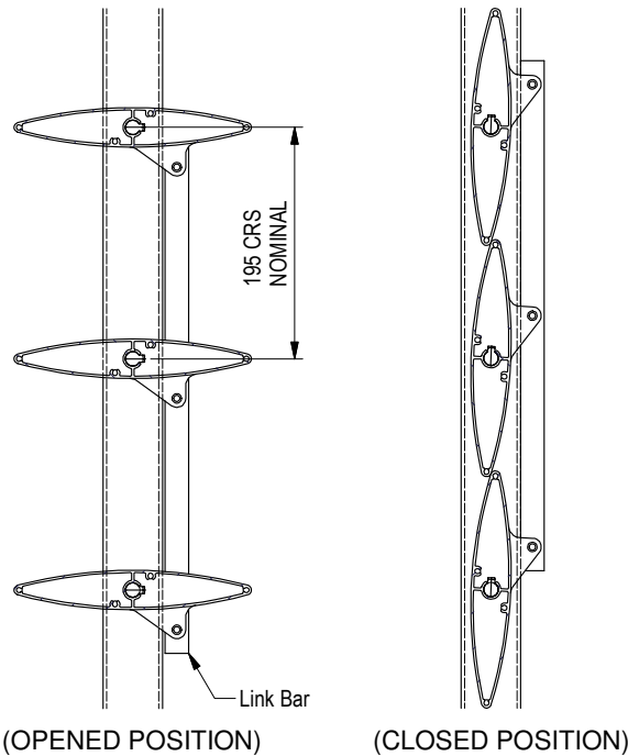
SECTIONED VIEW
