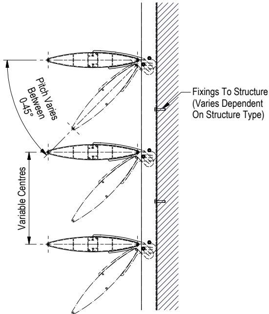
SECTIONED VIEW
