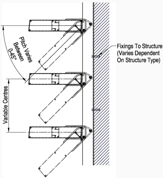
SECTIONED VIEW
