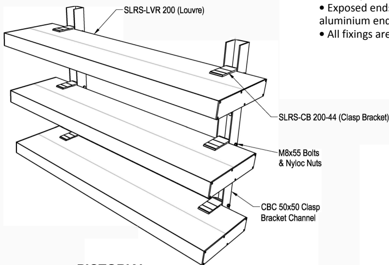
PICTORIAL
