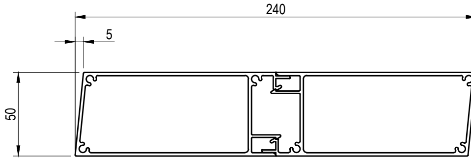
SLRS-LVR 240 - PROFILE
