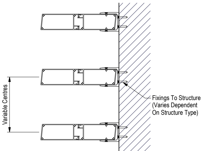
SECTIONED VIEW
