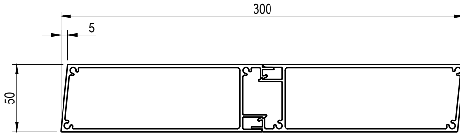
SLRS-LVR 300 - PROFILE
