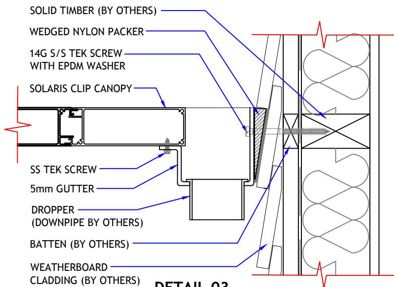
DETAIL 03
