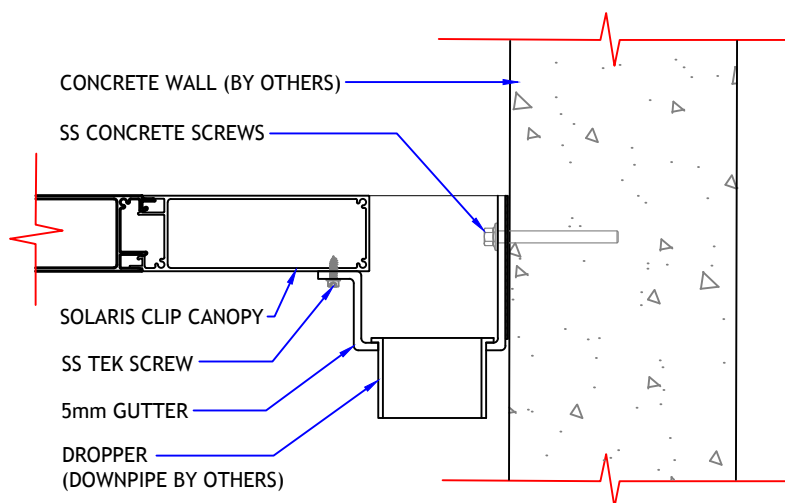
DETAIL 03
