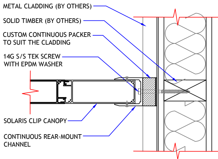
DETAIL 02
