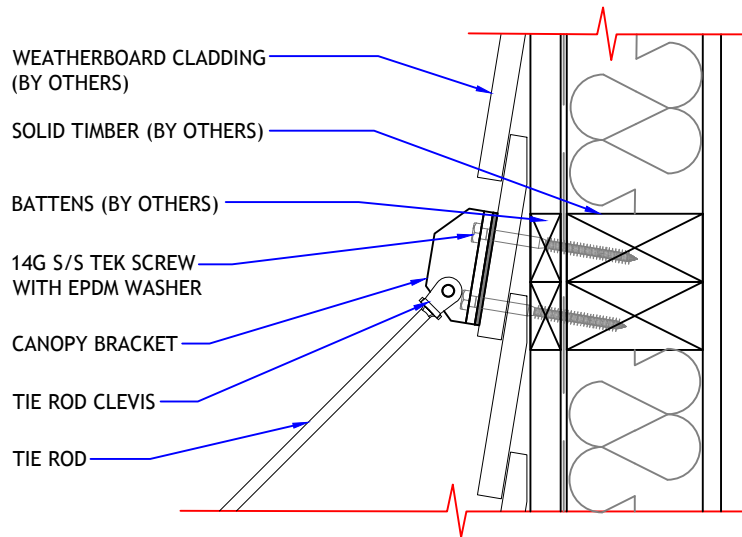
DETAIL 01
