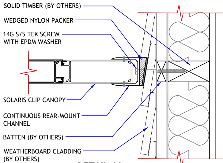
DETAIL 02
