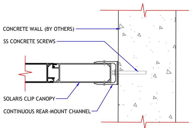
DETAIL 02
