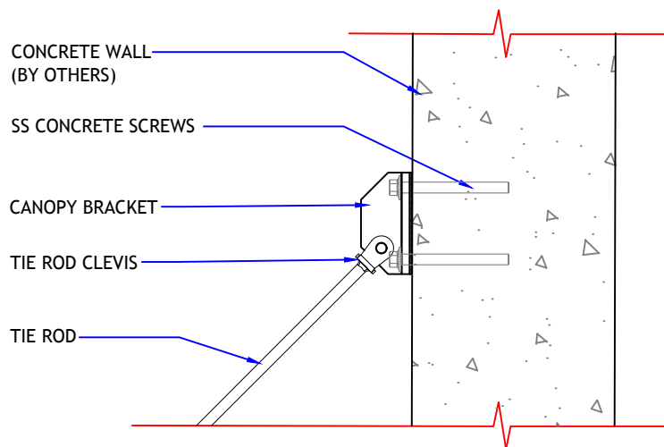
DETAIL 01
