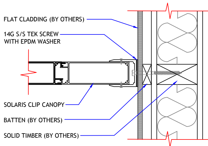
DETAIL 02
