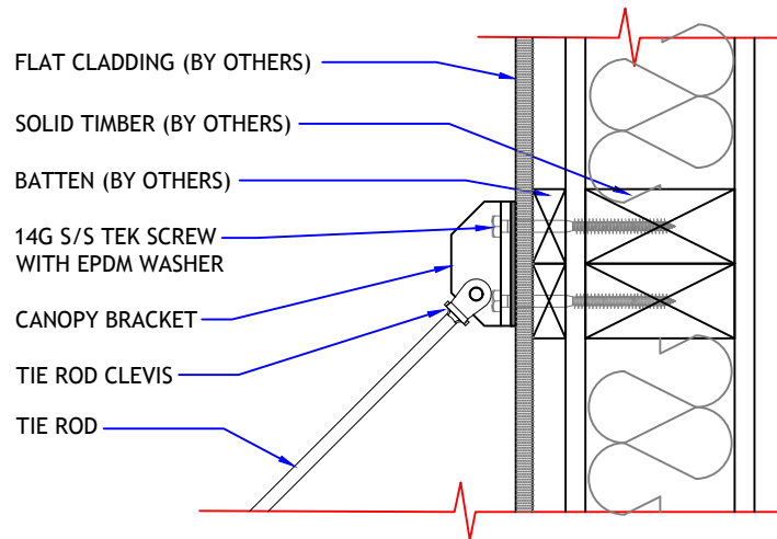
DETAIL 01
