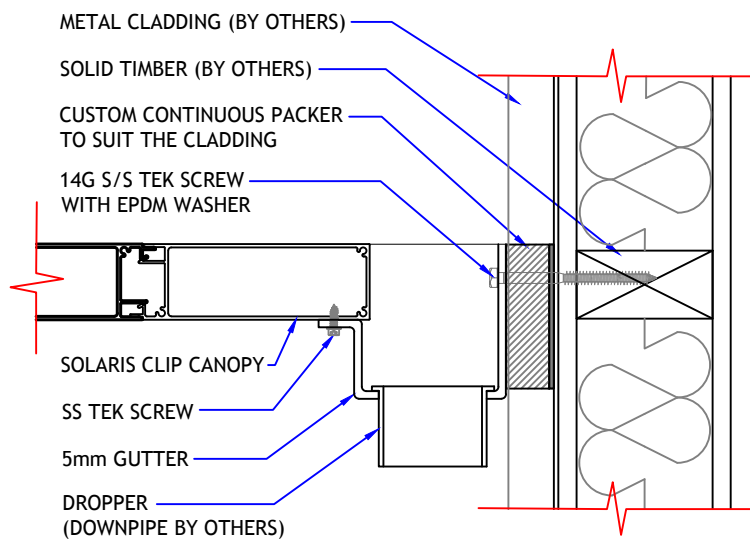
DETAIL 03
