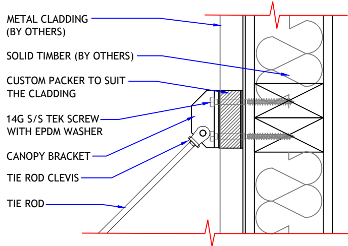
DETAIL 01
