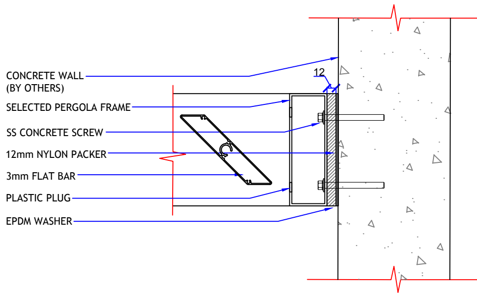
DETAIL 01 (Side View)
