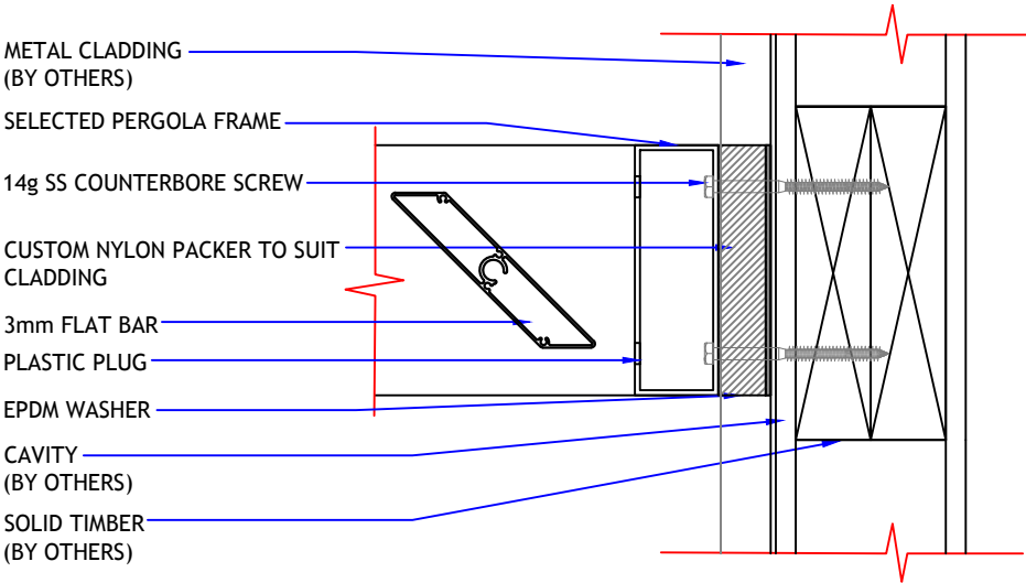
DETAIL 01 (Side View)
