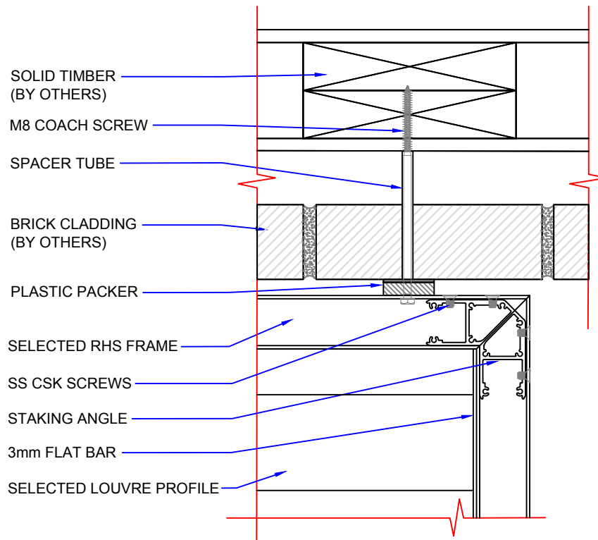
DETAIL 02 (Plan View)
