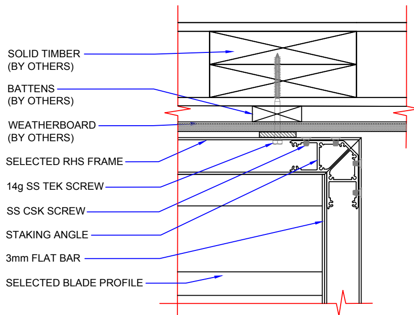
DETAIL 02 (Plan View)
