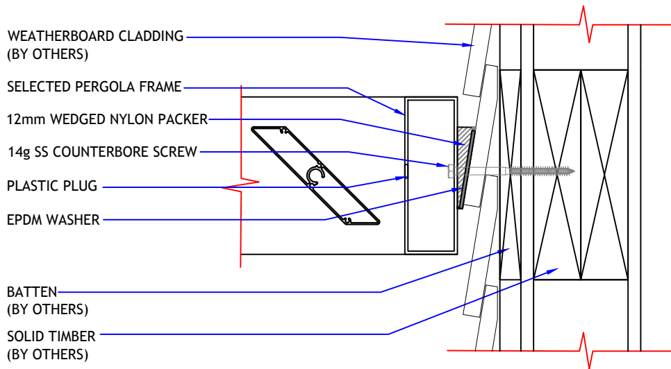
DETAIL 01 (Side View)
