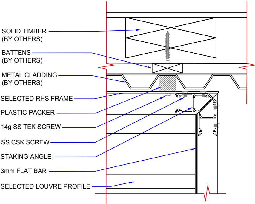
DETAIL 02 (Plan View)
