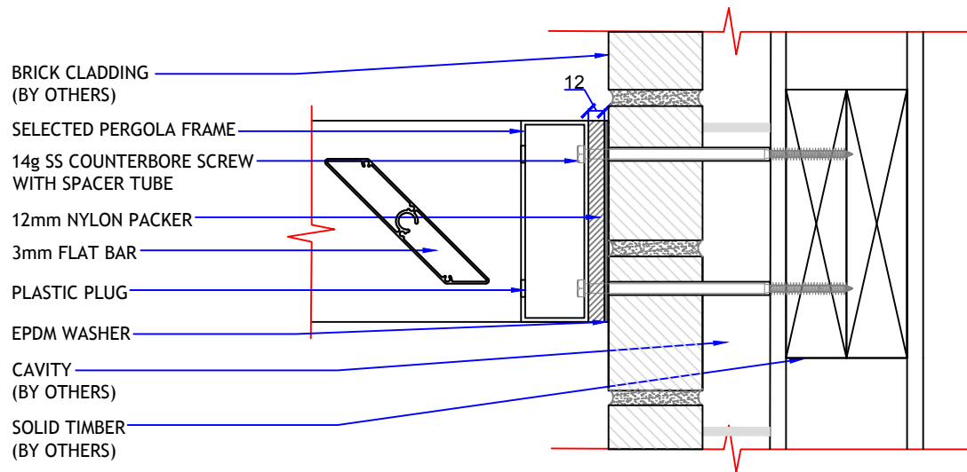
DETAIL 01 (Side View)
