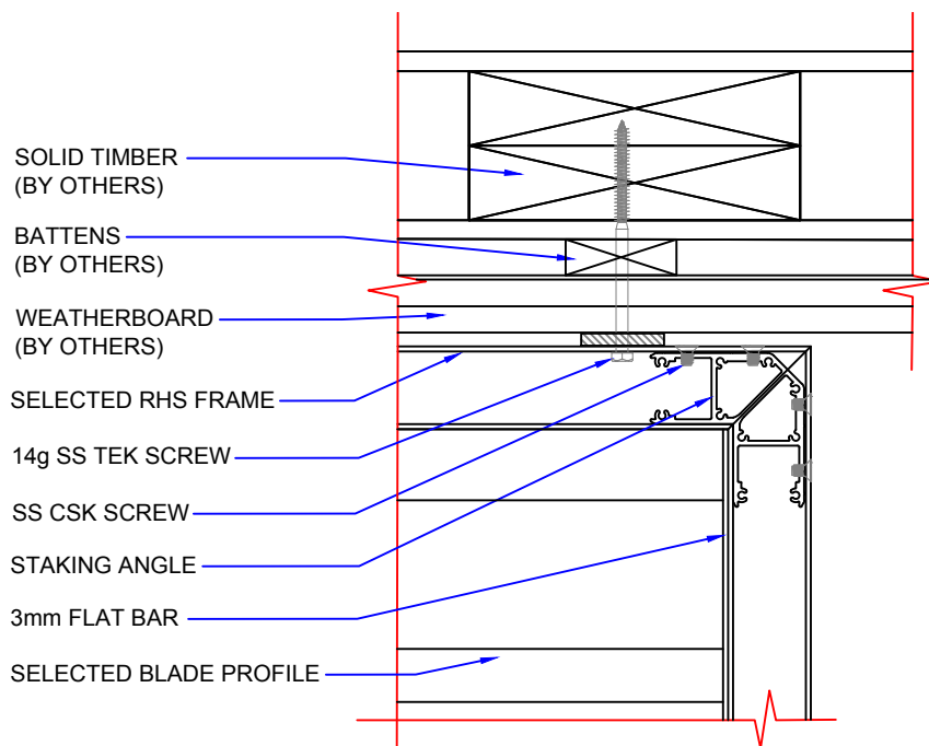
DETAIL 02 (Plan View)
