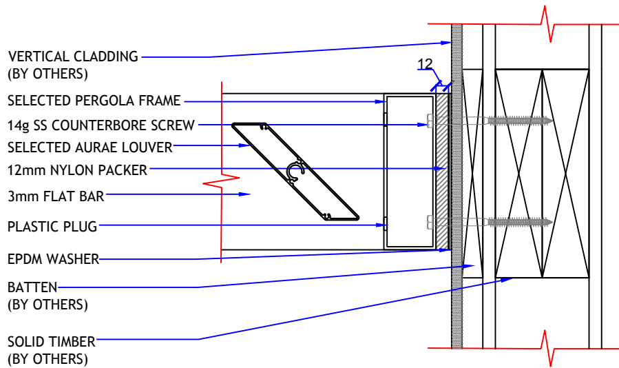
DETAIL 01 (Side View)
