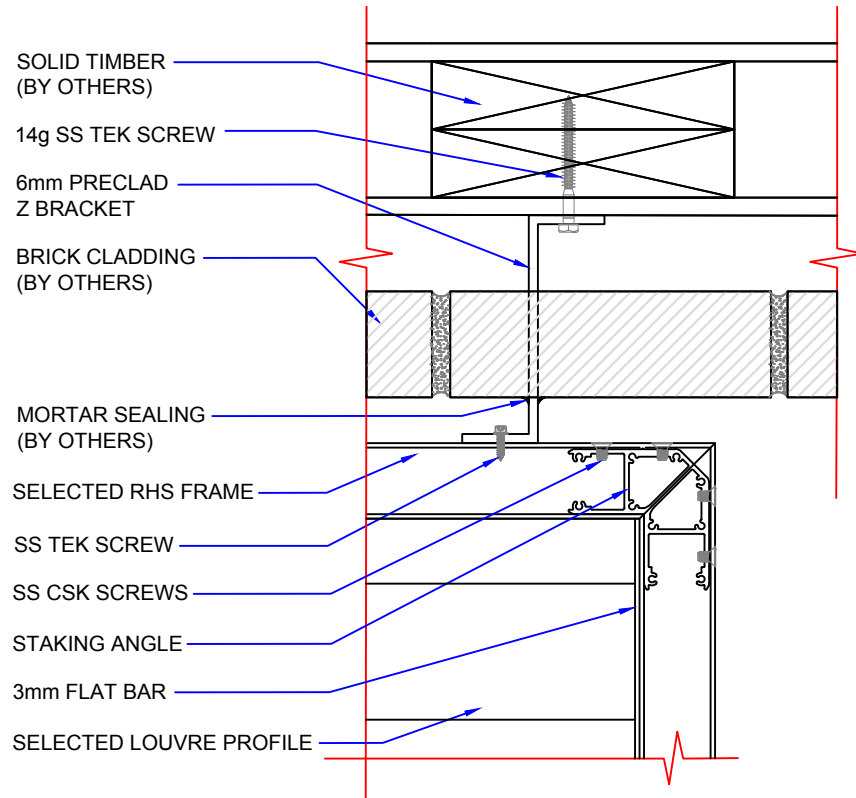
DETAIL 02 (Plan View)
