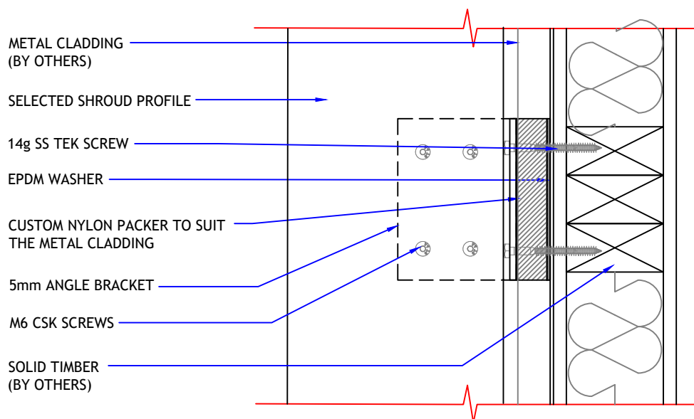
DETAIL 02 (Side View)
