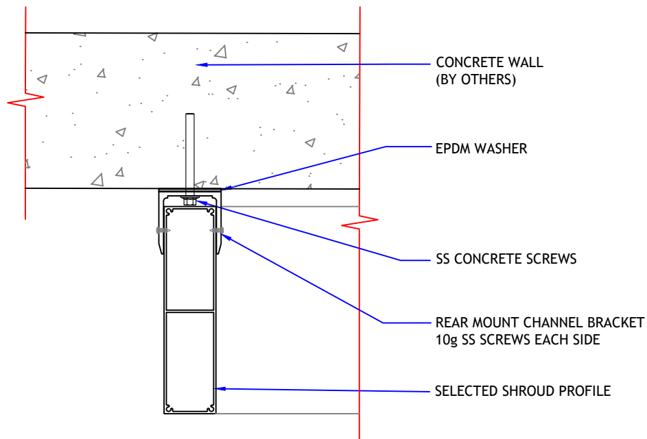
DETAIL 01 (Plan View)
