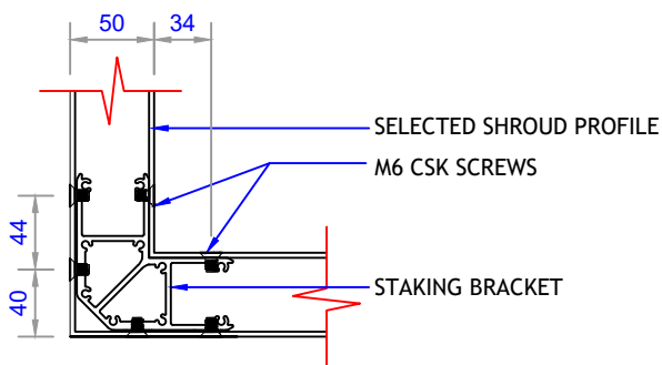
DETAIL 01
