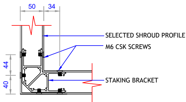
DETAIL 01
