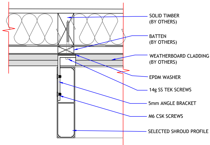
DETAIL 01 (Plan View)
