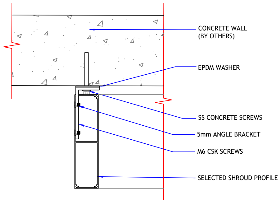
DETAIL 01 (Plan View)
