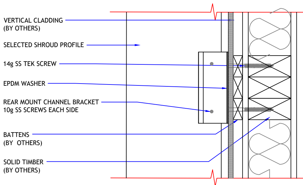
DETAIL 02 (Side View)
