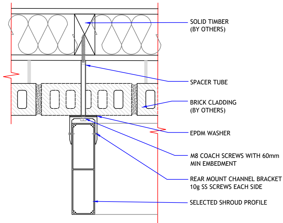
DETAIL 01 (Plan View)
