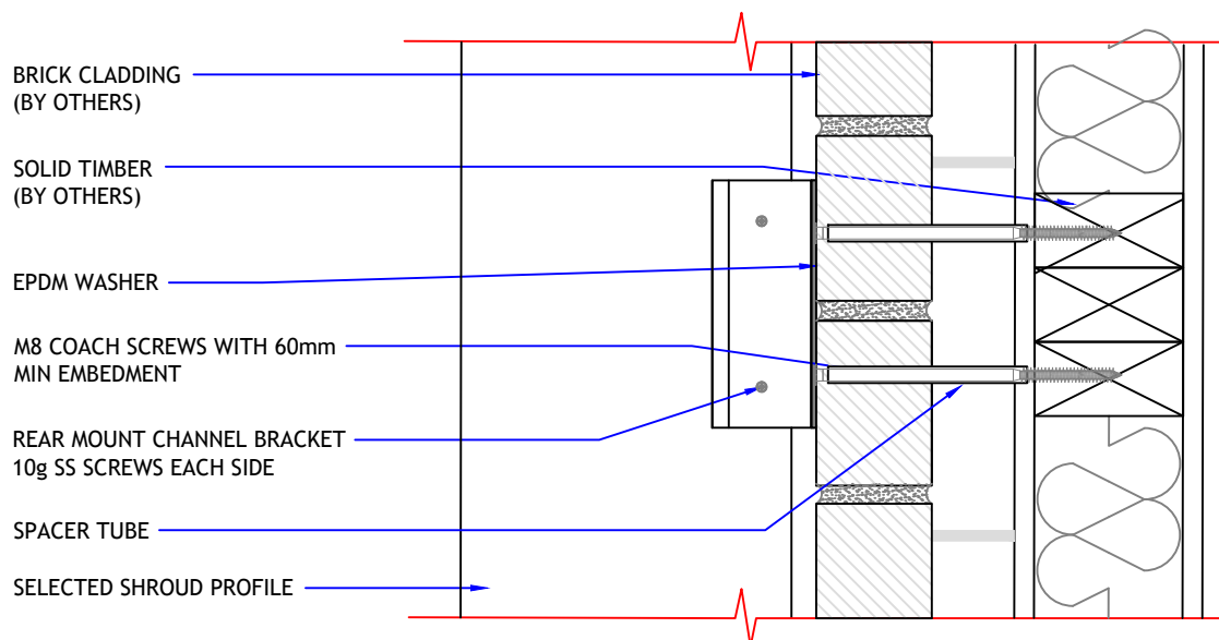
DETAIL 02 (Side View)
