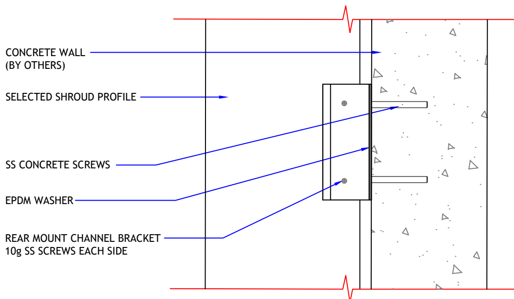
DETAIL 02 (Side View)
