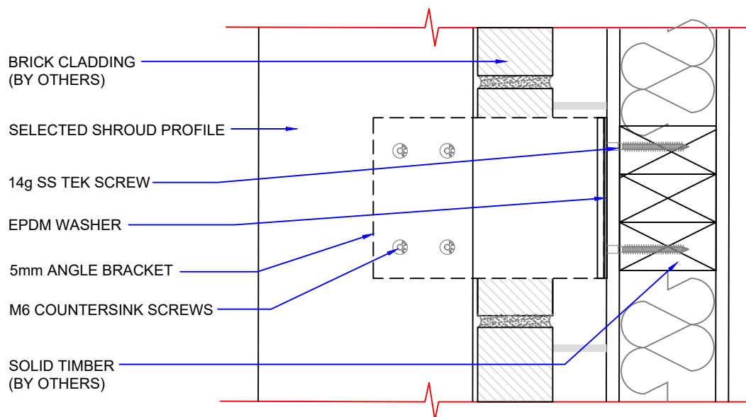
DETAIL 02 (Side View)
