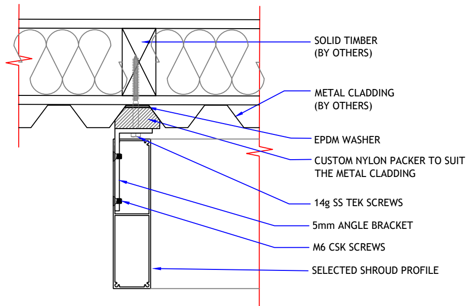
DETAIL 01 (Plan View)
