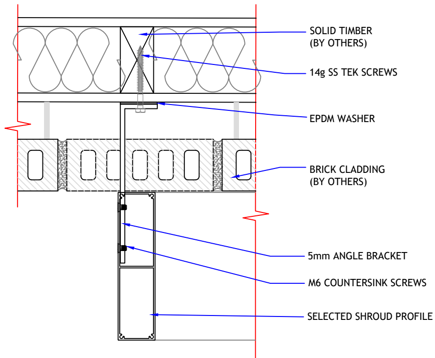
DETAIL 01 (Plan View)
